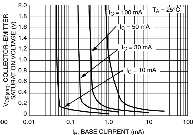
Figure 4. Saturation Region
